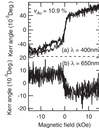
FIG. 4. Kerr loops of a film with v_{\text{Au}} = 10.9\% at wavelength of 400 nm (a) and 650 nm (b).
