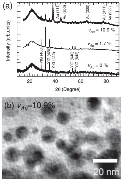
FIG. 1. (a) XRD profiles for films with v_{\text{Au}} = 0\% , 1.7%, and 10.9% annealed at 900 °C. (b) A cross-sectional TEM image of a film with v_{\text{Au}} = 10.9\% .
