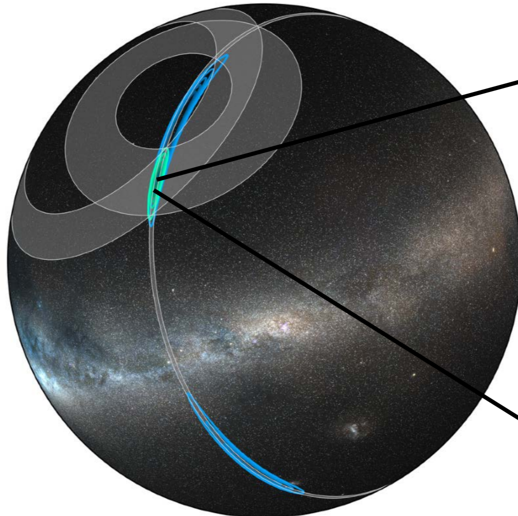
(C) LIGO/Virgo/NASA
